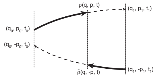
FIG. 1. Space-time coordinates for the forward and backward trajectories.
